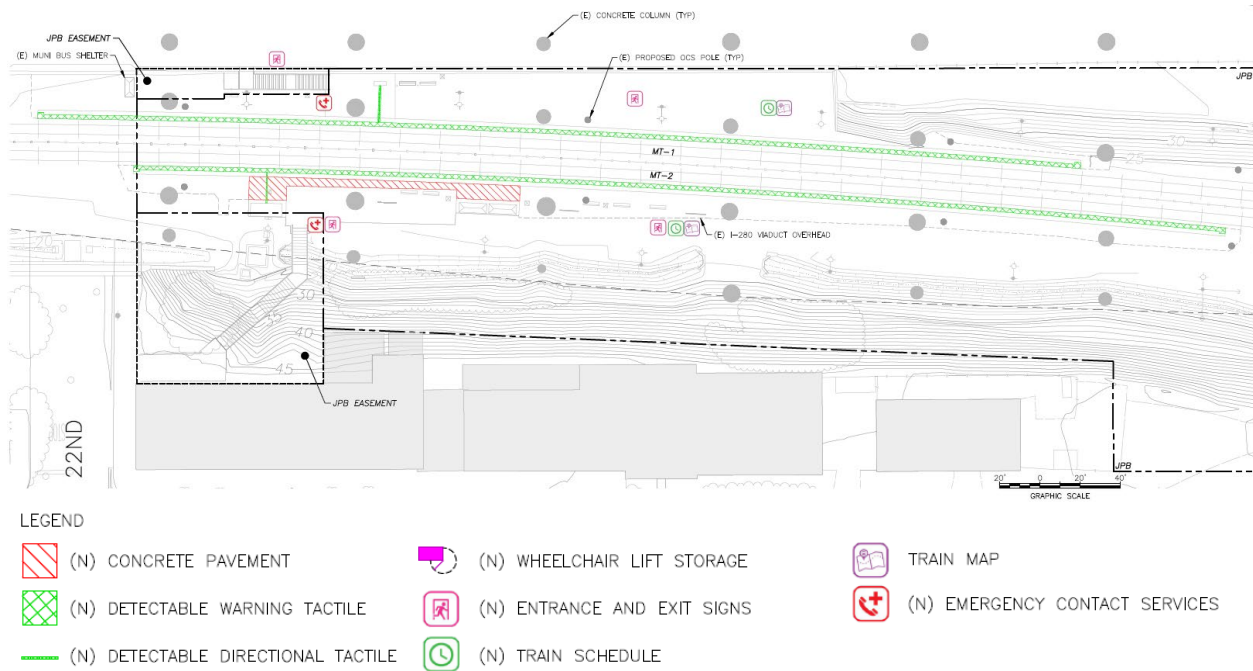
Figure 26 Non-Vertical Access Improvements Concept
