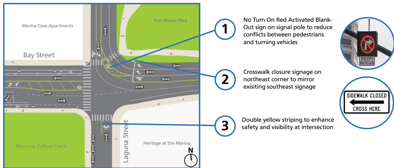
Figure 4-1. Quick-build proposals at Laguna Street / Bay Street
