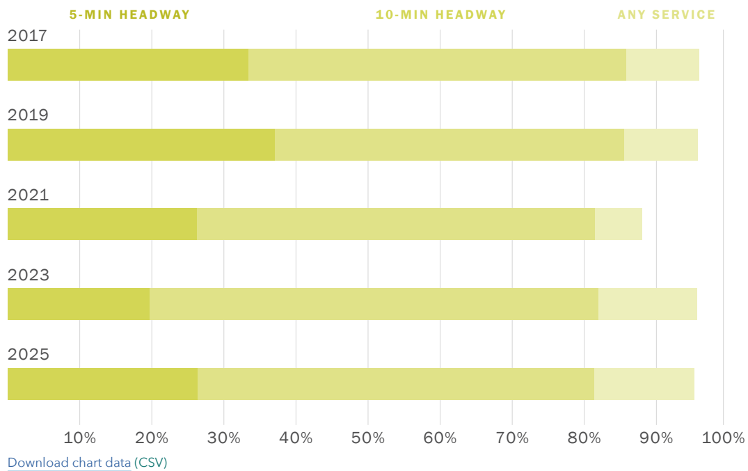
Figure 4-12. Percentage of SF Population Within a five-minute Walk of Muni Service by Service Frequency, Weekday PM Peak
