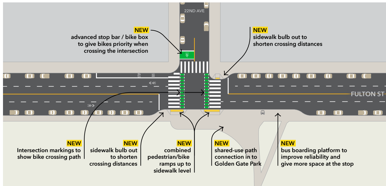
Figure 22. Fulton Street / 22nd Avenue Bike Connection Concept
