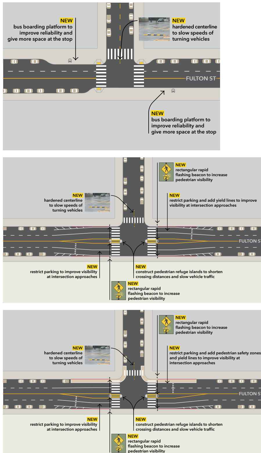
Figure 32. Example Intersection Treatments on Fulton Street
