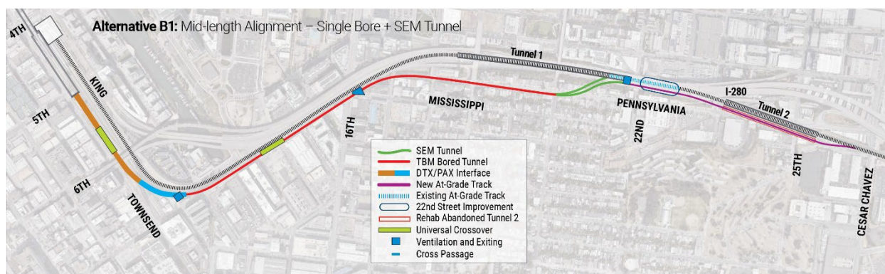
Figure 5-3. Fire/Life Safety Features for Mid-Length Alignment – Single Bore + SEM Tunnel
