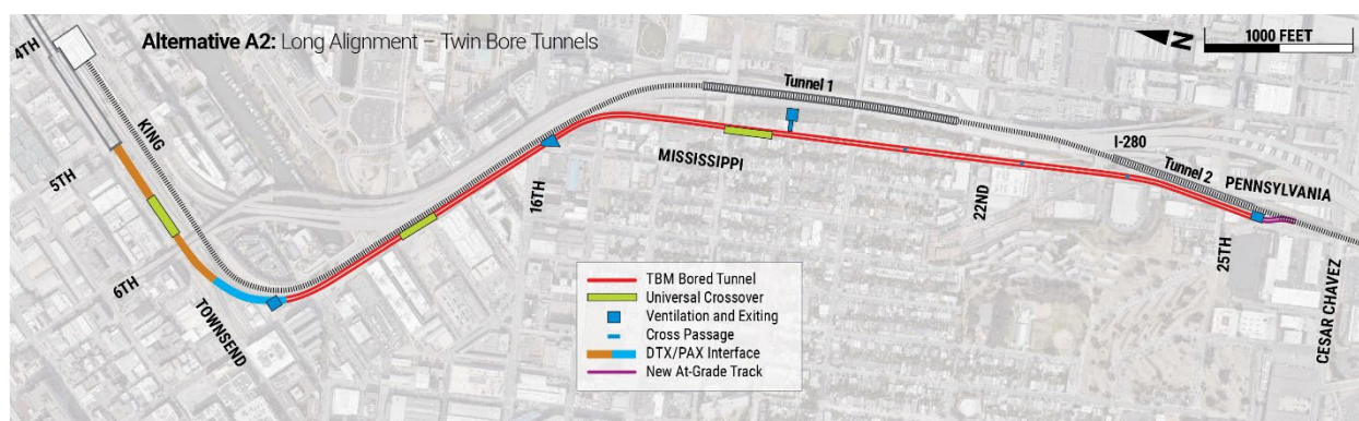
Figure 5-2. Fire/Life Safety Features for Long Alignment – Twin Bore Tunnels
