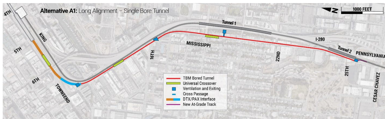
Figure 5-1. Fire/Life Safety Features for Long Alignment – Single Bore Tunnel
