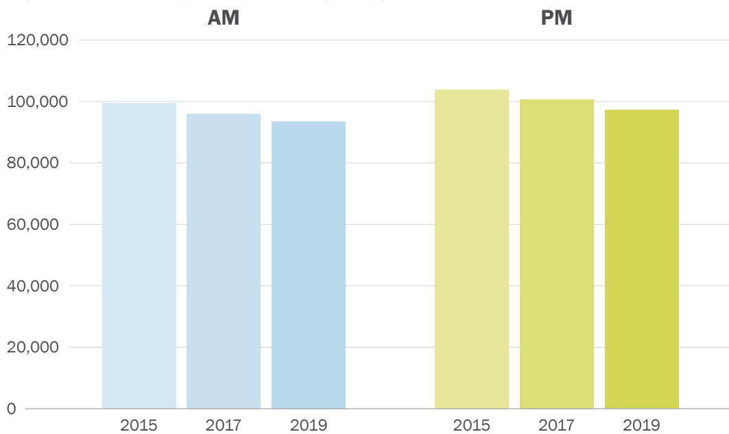
Figure 4-16: Weekday Mainline/Average Daily Traffic (ADT) Counts 2015 - 2019
