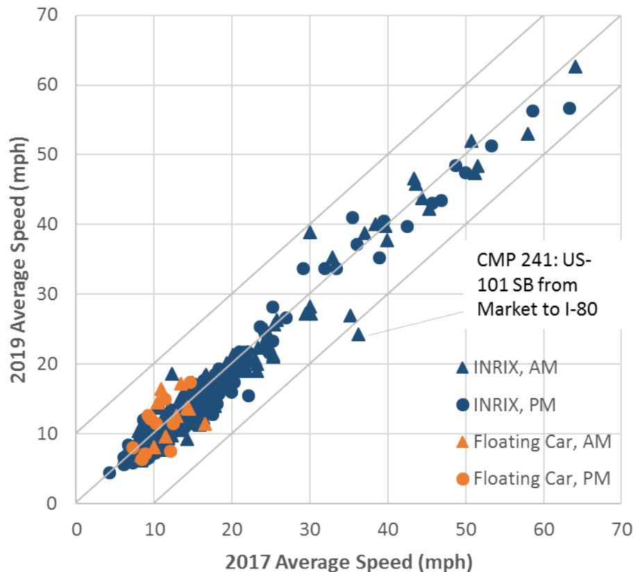
Figure A5-6: Comparison of 2017 and 2019 CMP Segment Speeds
