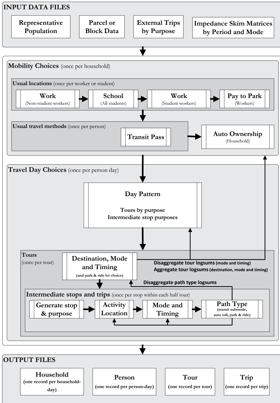
Figure A21-1: DaySim Model Components
