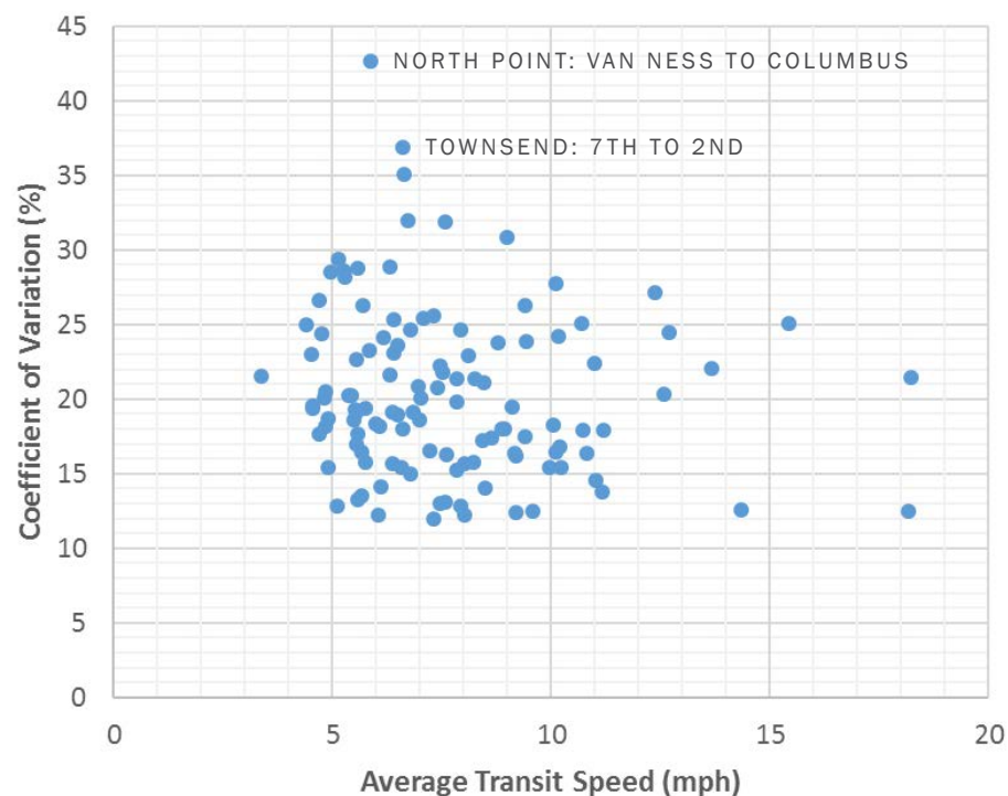
Figure A8-2: Reliability and Speed Matrix, PM Peak CMP Segment Reliability vs. Average Speed, PM Peak
