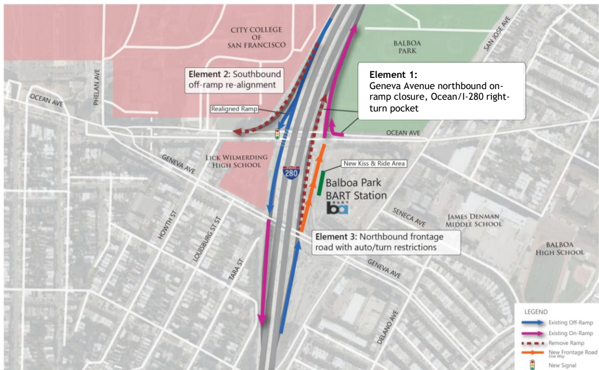
Figure ES-2: Alternative 1: Partial Split Interchange
