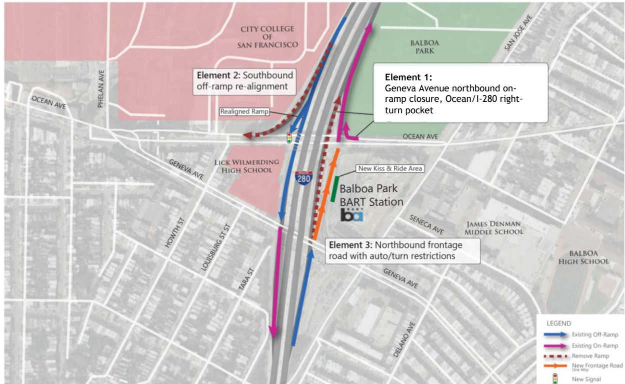
Figure 12: Alternative 1 Partial Split Interchange
